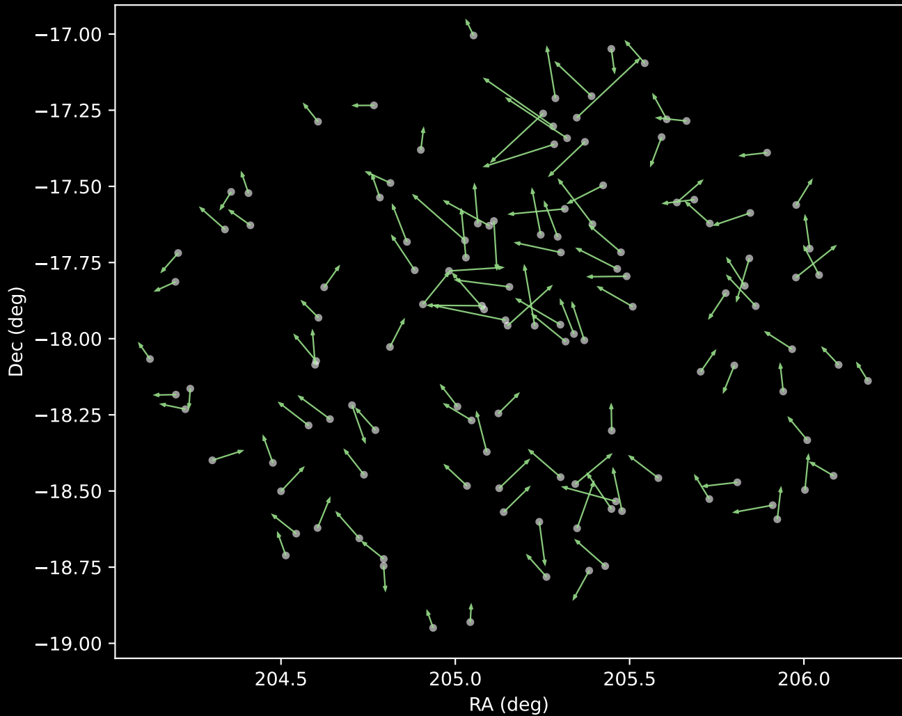
GALAH DR4 Cluster 5 Proper Motion Vectors (n=124)
