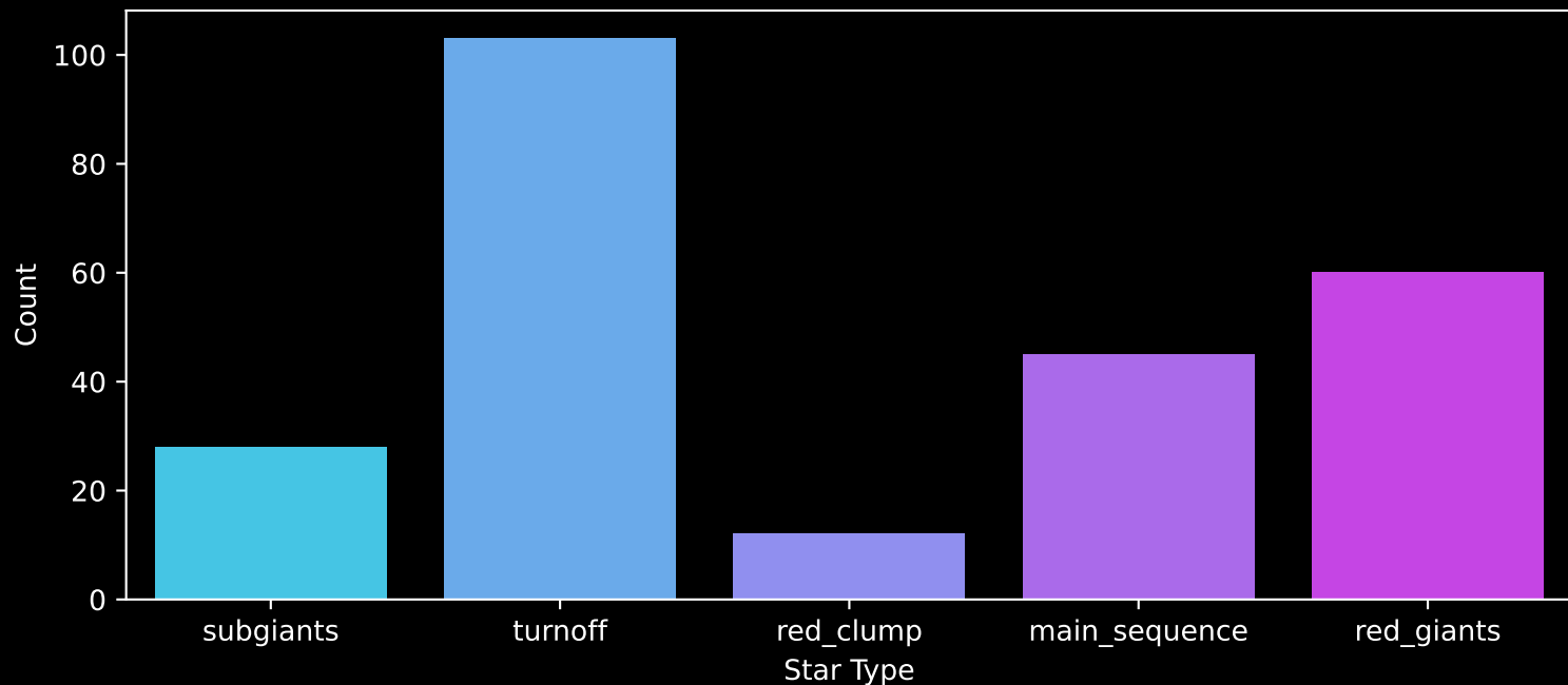
GALAH DR4 Field: [8615] Count plot of Star Type
