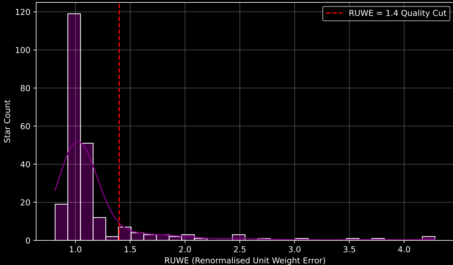
GALAH DR4 Field [8615] RUWE Distribution (n= 235)
